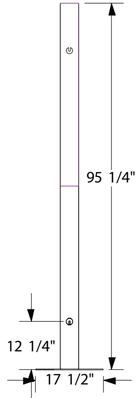
RIGHT VIEW
