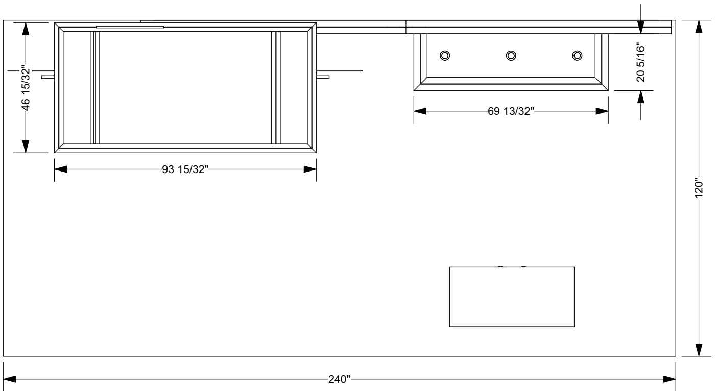
○ Plan View Scale 1:35
