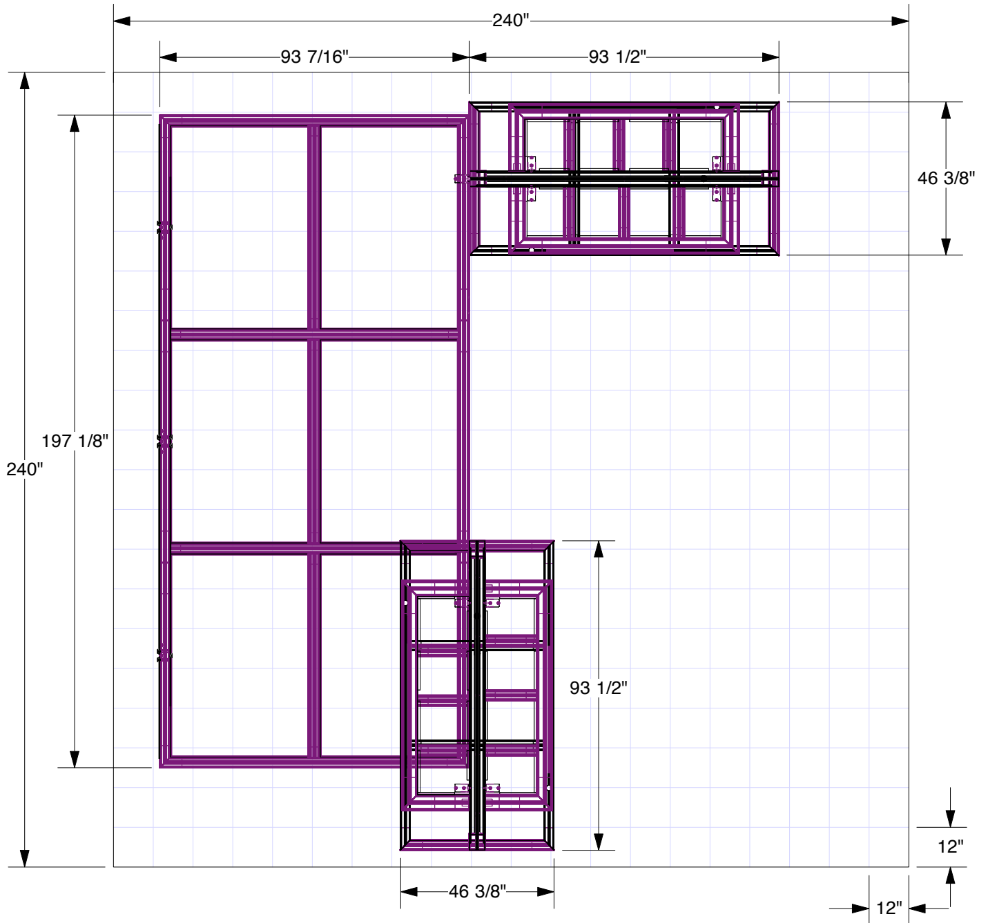
PLAN VIEW
