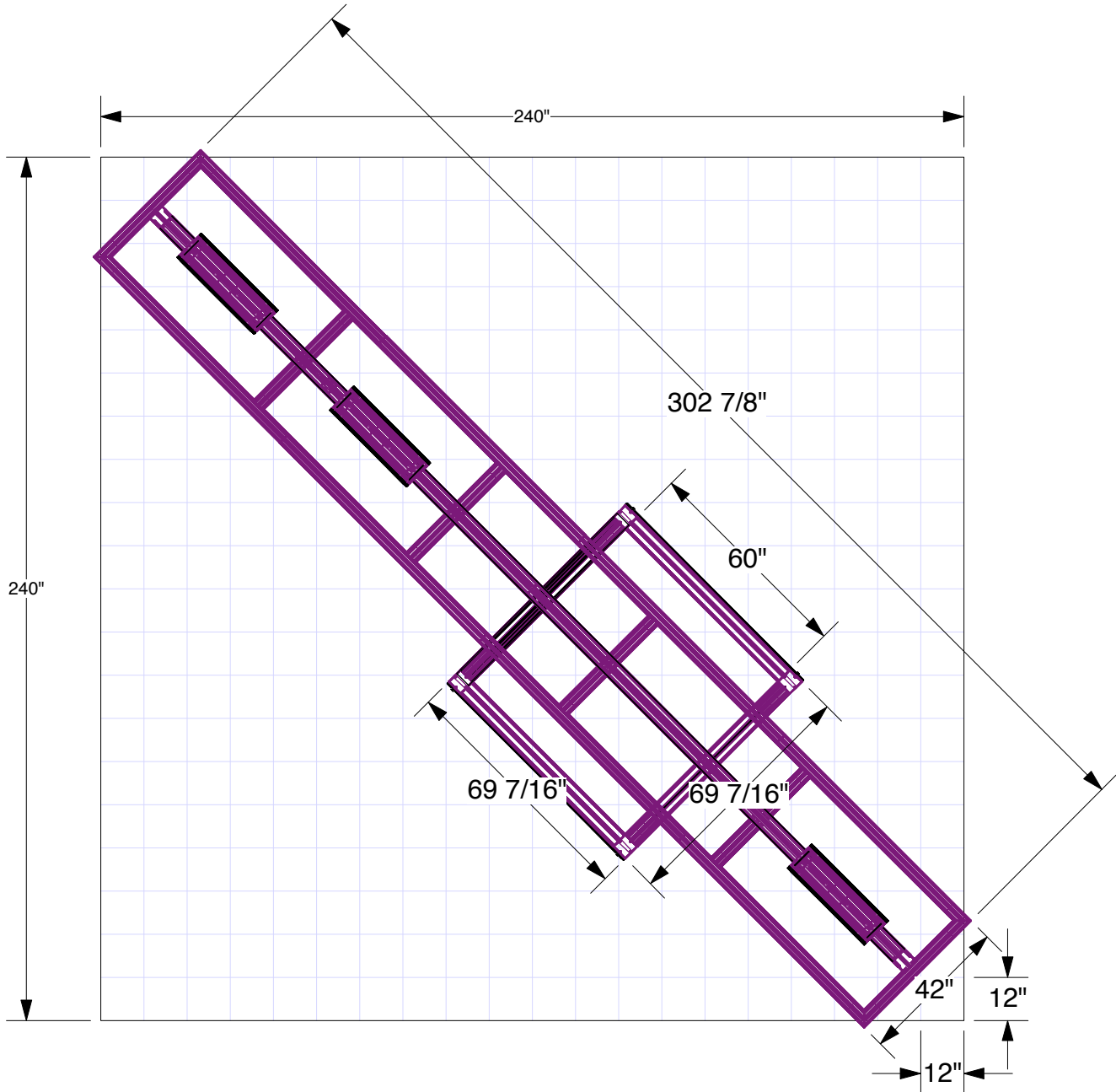
PLAN VIEW
