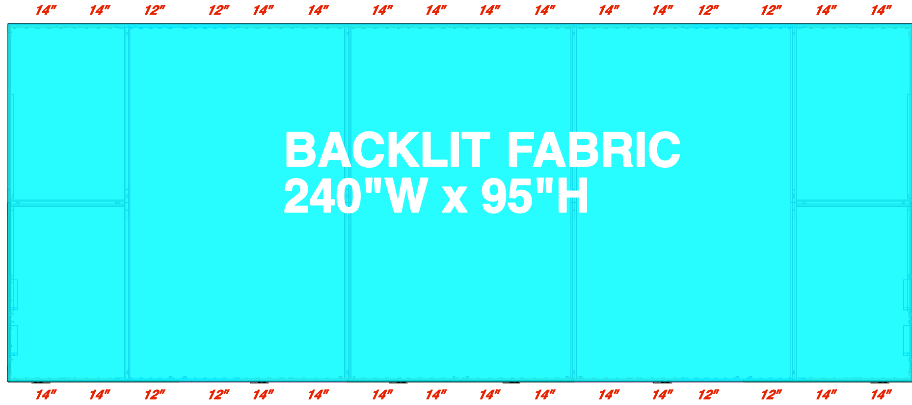
FRONT VIEW
