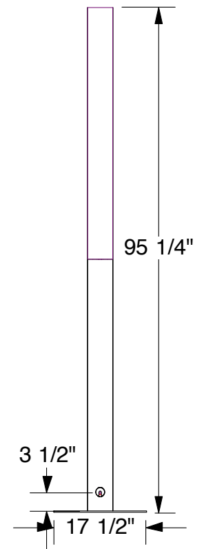
RIGHT VIEW
